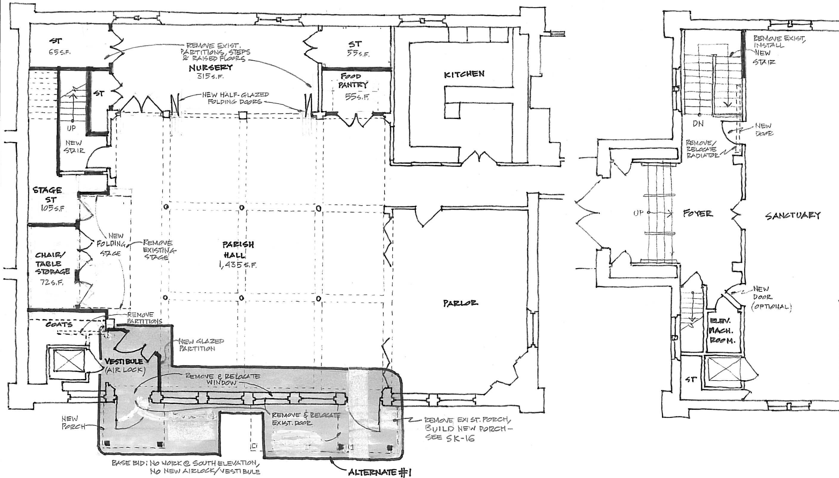
○ PART LOWER LEVEL PLAN @ PARISH HALL. OPTION "1" SCALE: 1/8" = 1'-0"
