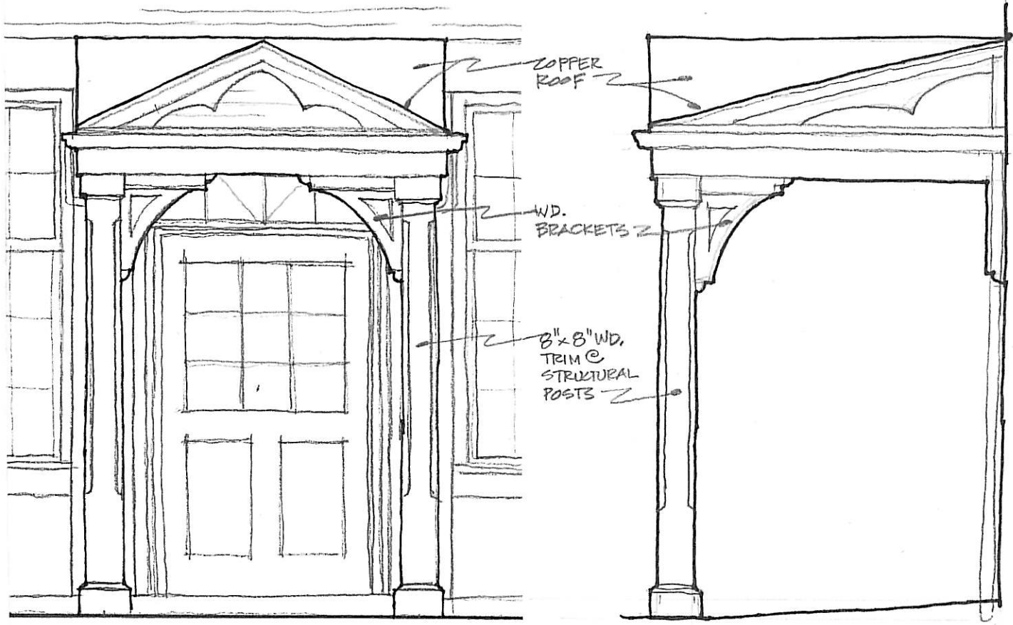
NEW PORCH. FRONT ELEVATION
