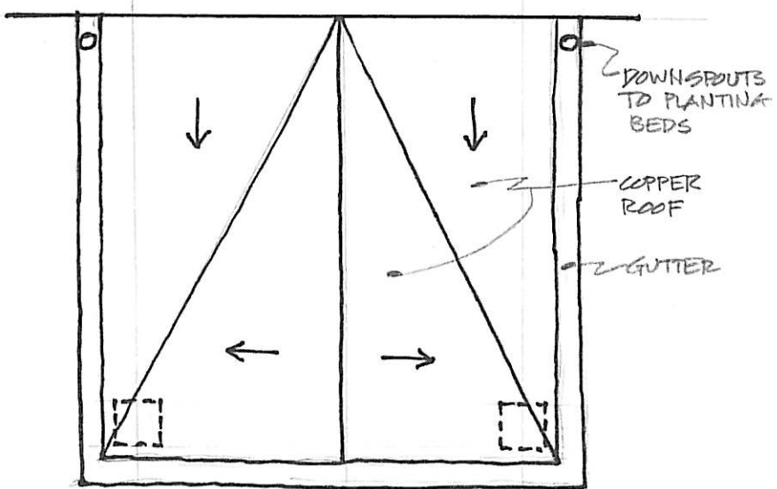
NEW PORCH. ROOF PLAN
